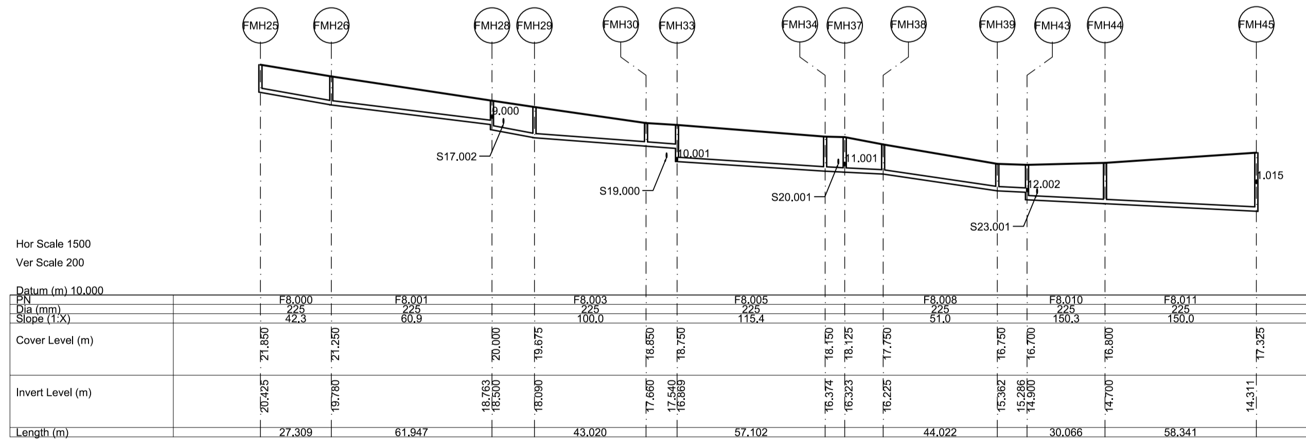
Longitudinal Section FMH25 - FMH45 Scale 1:1500 (Horizontally), 1:200 (Vertically)
