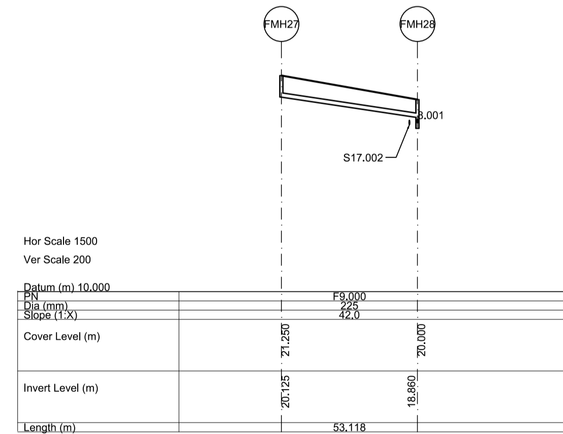
Longitudinal Section FMH27 - FMH28 Scale 1:1500 (Horizontally), 1:200 (Vertically)
