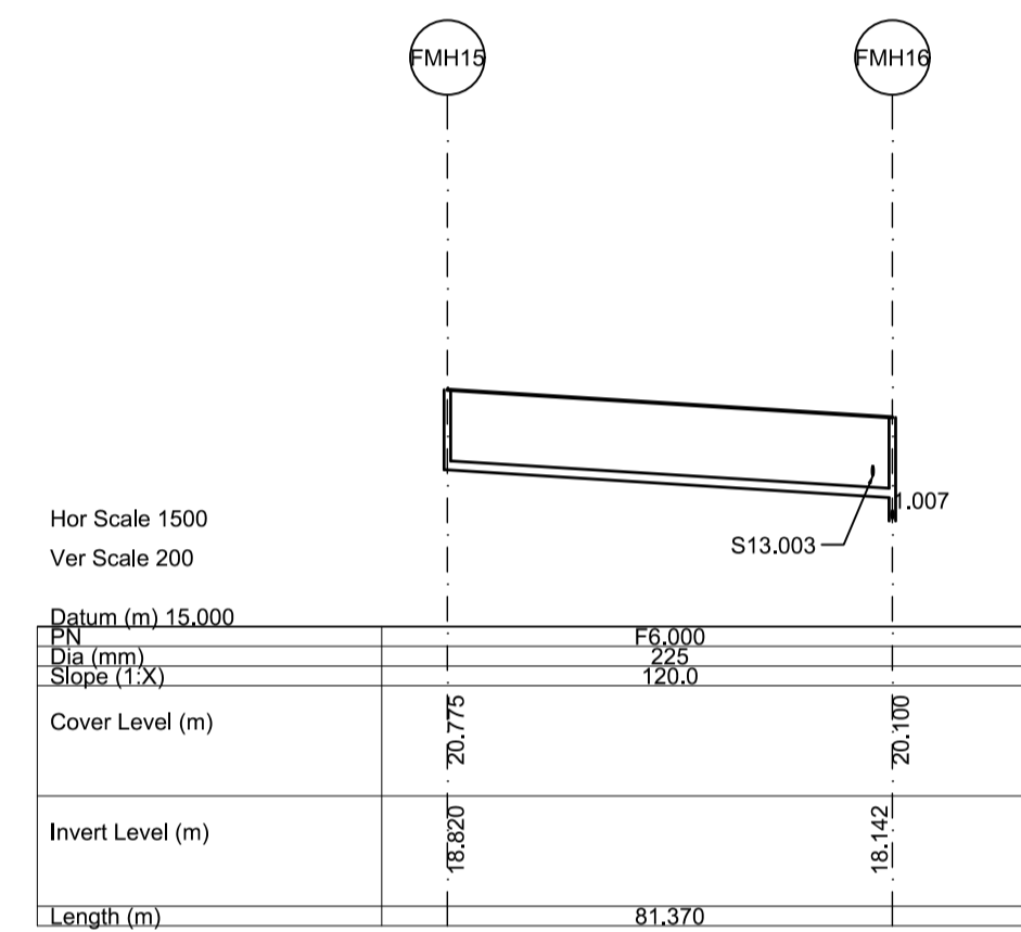
Longitudinal Section FMH15 - FMH16 Scale 1:1500 (Horizontally), 1:200 (Vertically)
