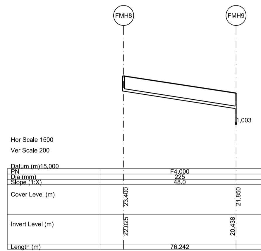
Longitudinal Section FMH8 - FMH9 Scale 1:1500 (Horizontally), 1:200 (Vertically)
