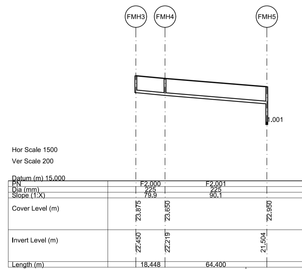
Longitudinal Section FMH3 - FMH5 Scale 1:1500 (Horizontally), 1:200 (Vertically)
