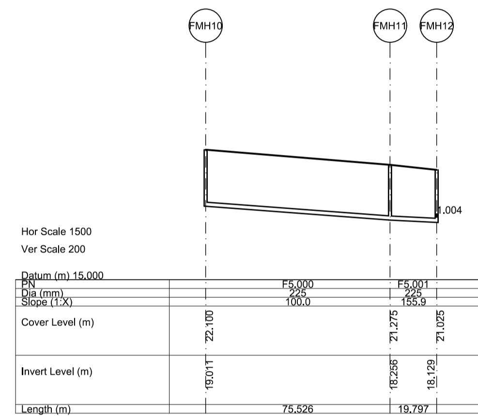
Longitudinal Section FMH10 - FMH12 Scale 1:1500 (Horizontally), 1:200 (Vertically)
