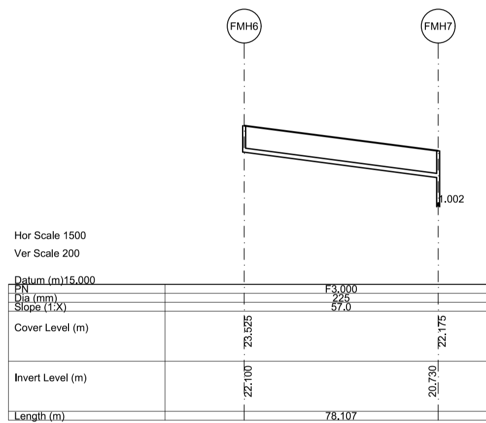
Longitudinal Section FMH6 - FMH7 Scale 1:1500 (Horizontally), 1:200 (Vertically)
