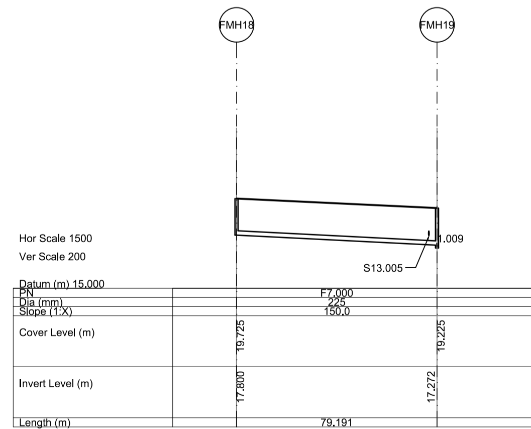
Longitudinal Section FMH18 - FMH19 Scale 1:1500 (Horizontally), 1:200 (Vertically)
